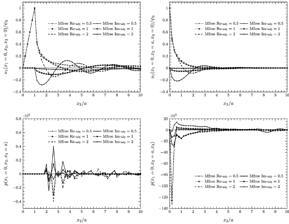
FIGURE 13 The transversely isotropic poroelastic half-space subjected to the torsion disk vibration.
