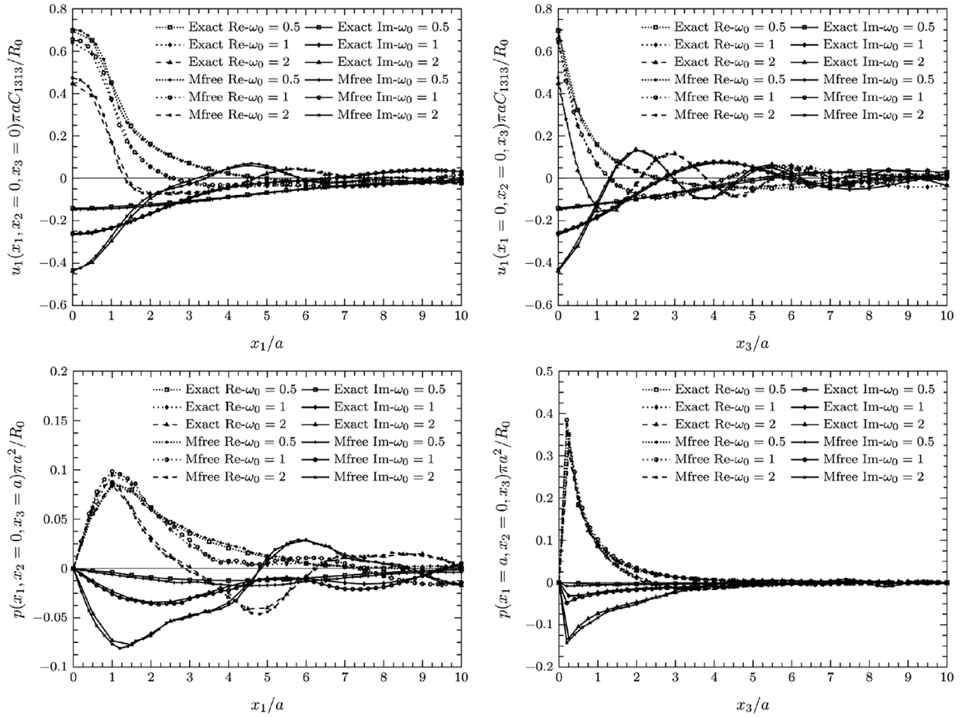
FIGURE 6 The transversely isotropic poroelastic half-space subjected to circular uniform horizontal force.
