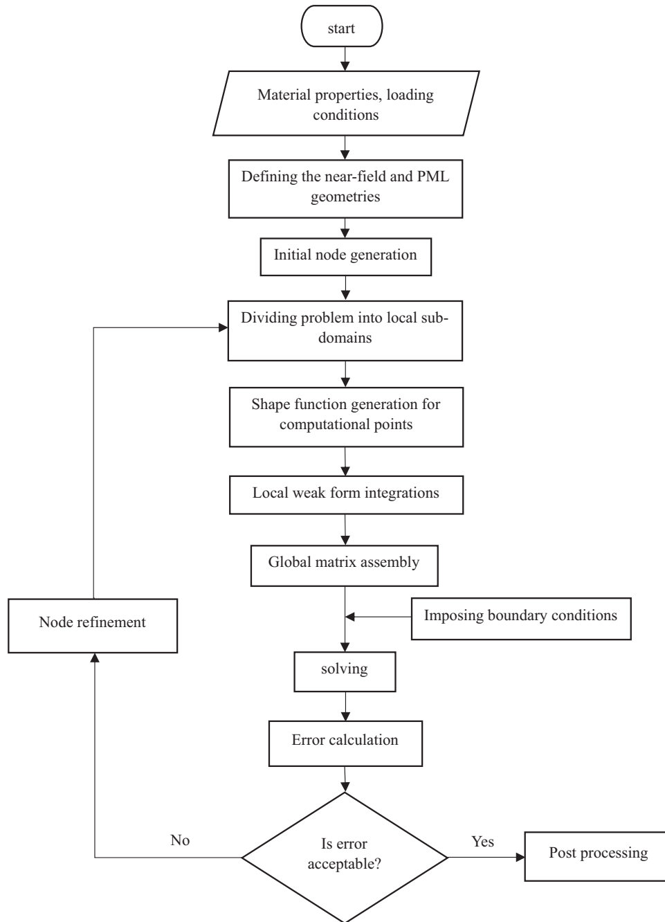
FLOW CHART 1 The steps to perform the PML based MLPG method. MLPG, meshless local Petrov–Galerkin; PML, perfectly matched layer.
