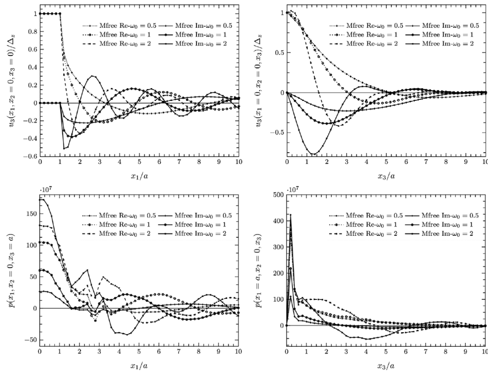
FIGURE 11 The transversely isotropic poroelastic half-space subjected to the vertical disk vibration.
