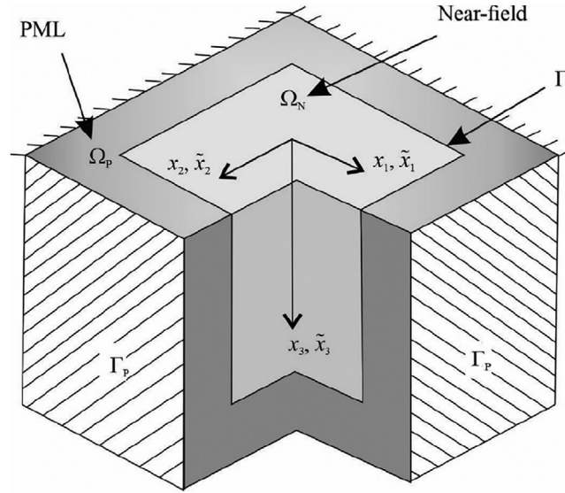
FIGURE 3 The near field and the PML in the stretched coordinate system. PML, perfectly matched layer.
