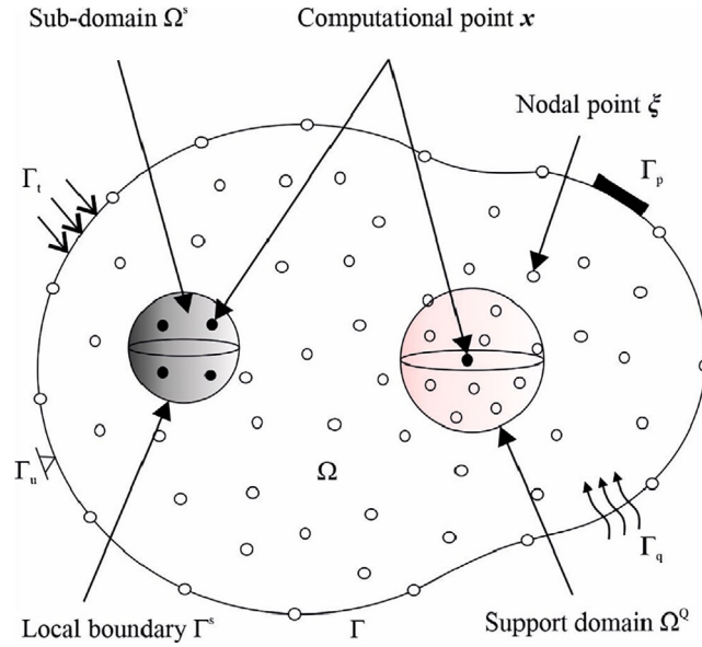
FIGURE 4 \Omega^s and \Gamma^s are the local subdomain and its boundary, which are used for the weak form integration. The support domain \Omega^Q corresponding to the computational point \mathbf{x} is used for constructing the shape functions. Different BCs are also shown. BCs, boundary conditions.
