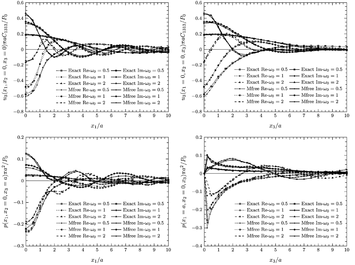
FIGURE 7 The transversely isotropic poroelastic half-space subjected to circular uniform vertical force.
