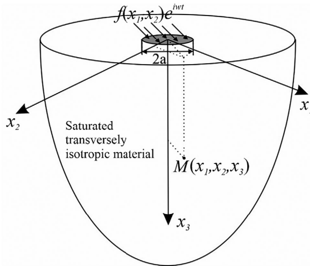
FIGURE 1 The half-space containing saturated transversely isotropic materials in both mechanical and hydraulic points of view subjected to arbitrary BCs. BCs, boundary conditions.
