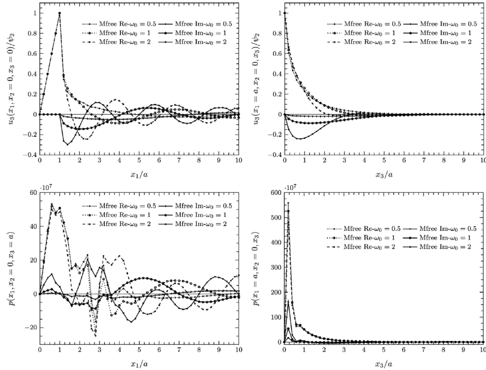
FIGURE 12 The transversely isotropic poroelastic half-space subjected to the rocking disk vibration.
