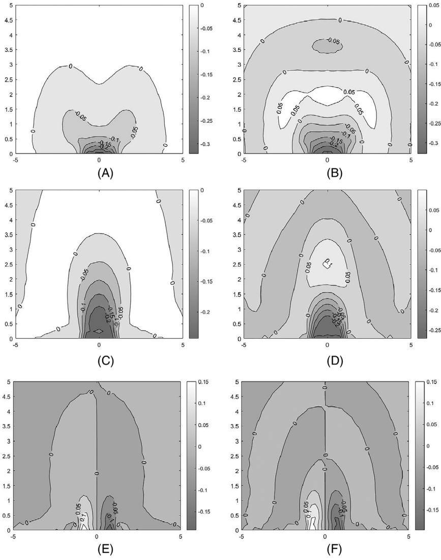
FIGURE 9 The iso-stress curves in x_1x_3 -plane for the half-space subjected to the uniform horizontal patch load (A) \sigma_{rz} , w_0 = 1 and (B) \sigma_{rz} , w_0 = 2 , the uniform vertical patch load (C) \sigma_{zz} , w_0 = 1 and (D) \sigma_{zz} , w_0 = 2 , and the rocking patch load (E) \sigma_{zz} , w_0 = 1 and (F) \sigma_{zz} , w_0 = 2 .
