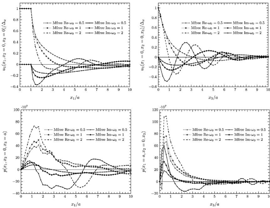
FIGURE 10 The transversely isotropic poroelastic half-space subjected to the horizontal disk vibration.
