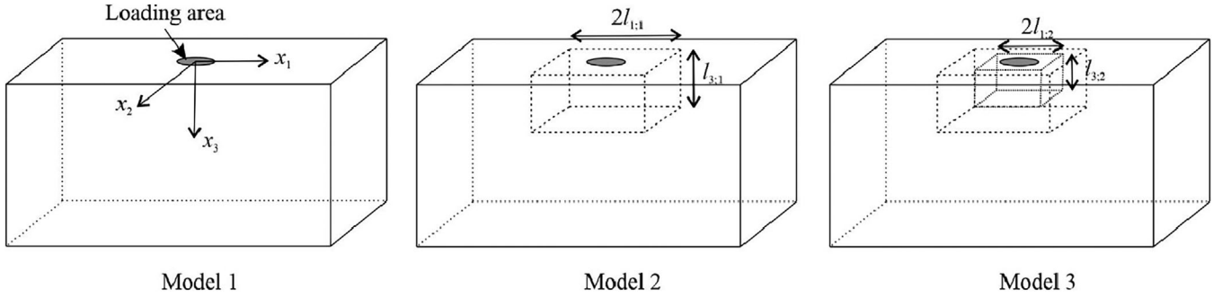
FIGURE 5 Refinement of nodes around the loading area for improving the meshless analysis results. Model1: uniform node distribution, Model 2: adding some nodes to Model 1 in the specific region, and Model 3: adding some further nodes to Model 2 in the specific region.
