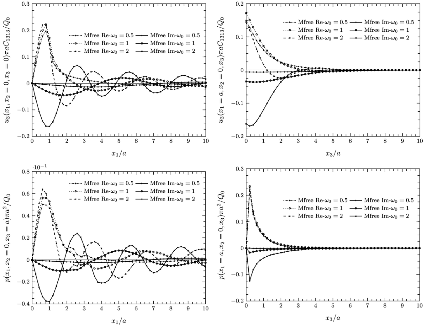
FIGURE 8 The transversely isotropic poroelastic half-space subjected to circular rocking force.
